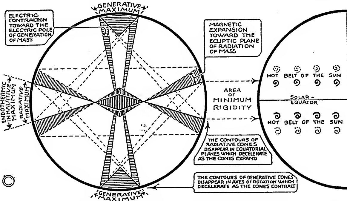
CHART No. 1. THE BREATHING OF THE SUN. EXPLAINING THE PERIODIC SHIFTING OF SUN-SPOTS IN CONFORMITY WITH THE CHANGING MAGNETIC BASES AND ECLIPTIC PLANE OF THE SUN
